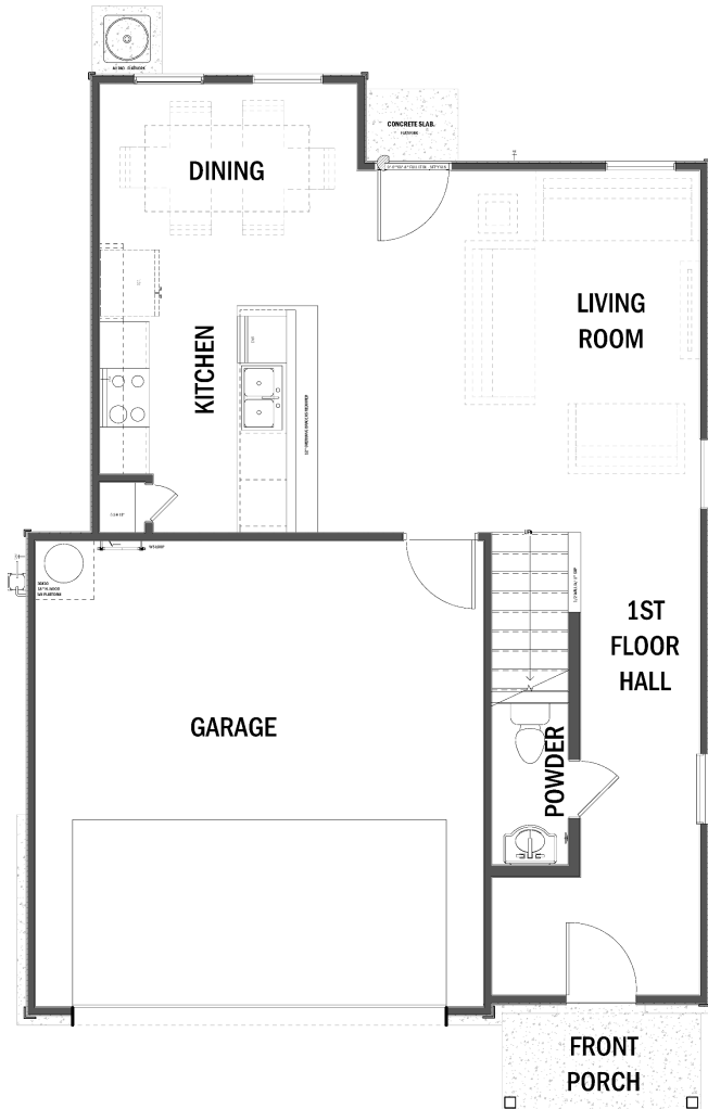
1st Floor
