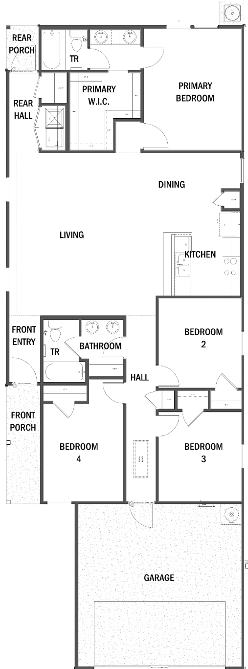
Floor Plan
