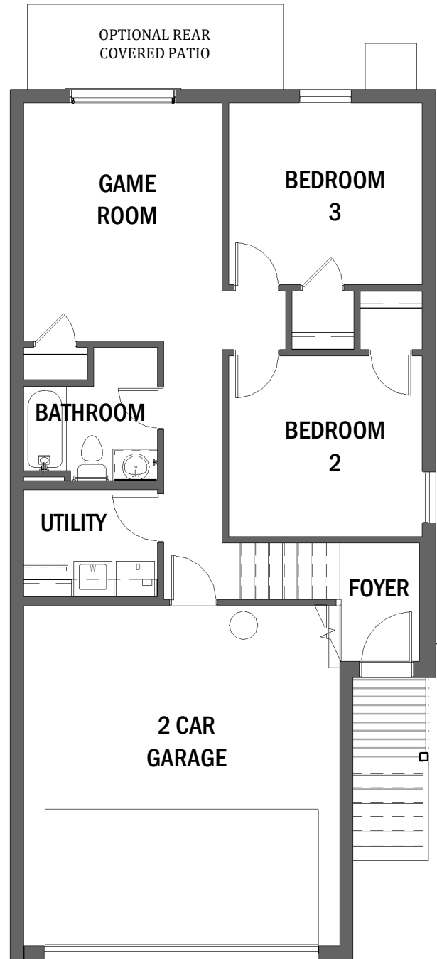
1ST FLOOR
